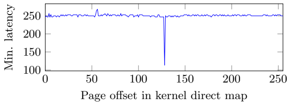
Figure 3: Minimum memory access time for an address p after prefetching different inaccessible addresses, on an i5-3320M. Peak shows the single address \bar{p} mapping to the same physical address as p .
