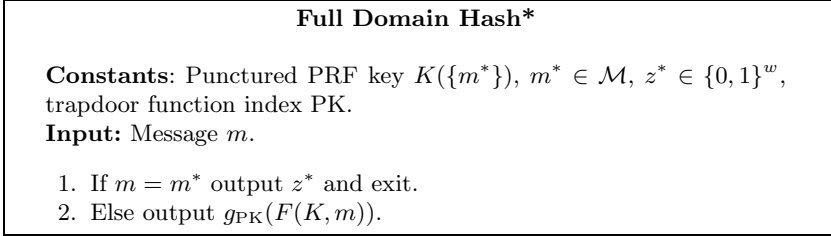
Fig. 2. Full Domain Hash*
