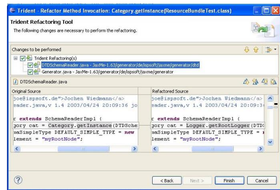
Figure 4. Trident reference refactoring preview.
