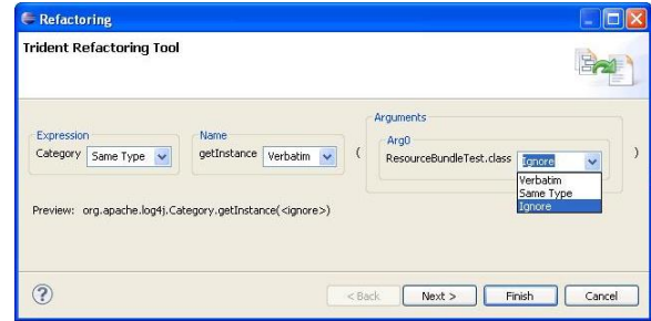
Figure 1. Trident search configuration.
