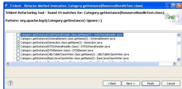
Figure 2. Trident search results.
