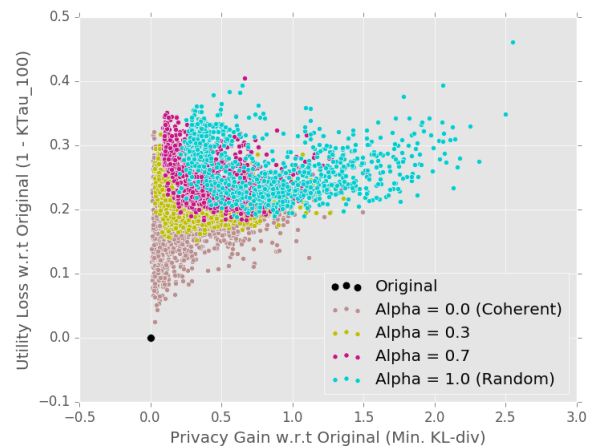
Figure 3: Empirical measures per user (search).
