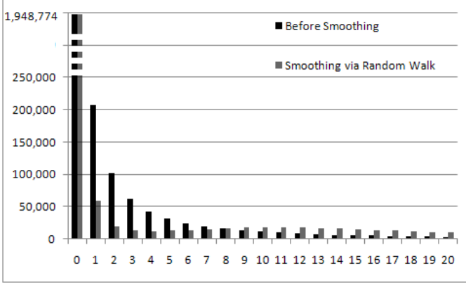
Figure 4. Length distribution of the clickthrough streams (with \text{StreamLength}_q \leq 20 ) in the Japanese training data, where x-axis is the stream length, and y-axis is the number of training samples; Bars at x = 0 shows the number of documents without click. Black bars correspond to the raw click counts and grey bars to the smoothed counts using Random Walk.
