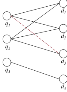
Figure 5. Before expansion, document d_3 has a clickthrough stream consisting of query q_2 only; after expansion, the clickthrough stream is augmented with query q_1 which has a similar click pattern as q_2 .
