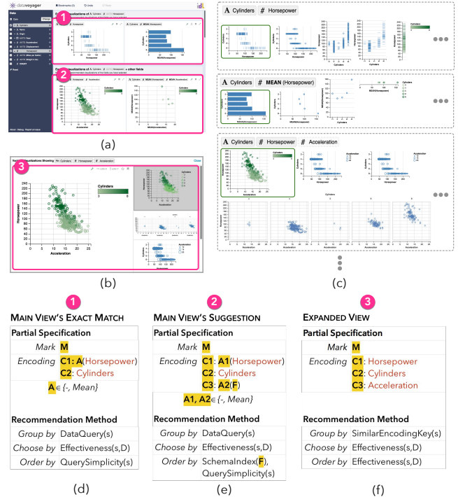
Figure 8: Voyager [25]. (a) The Main View shows visualizations with different data queries, promoting exploration of different fields. The Exact Match section contains all and only the selected fields. The Suggestion section contain all selected fields and one extra field to encourage further exploration. (b) The Expanded View displays various encodings of the same data query. (c) Groups of enumerated visualizations. The Main View only displays the top item from each group (highlighted with green border). (d-f) CompassQL queries for different sections.
