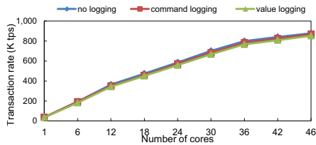
Figure 16: Transaction rate with different logging mechanisms. The number of warehouses is set to 12.
