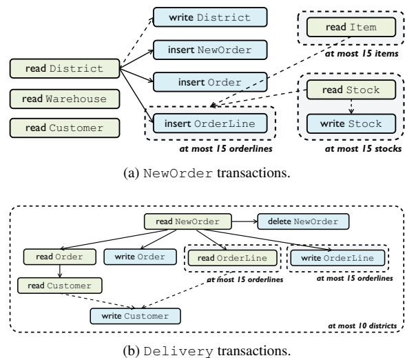
Figure 15: Program dependency graphs.
