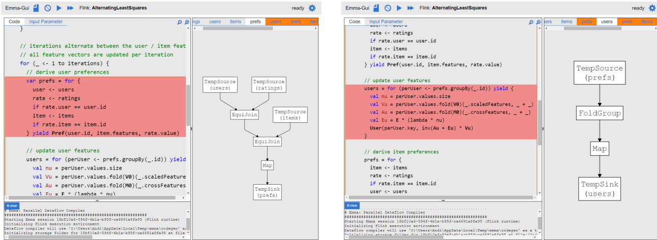
Figure 2: Two stages in the execution of an Alternating Least Squares algorithm in Emma.
