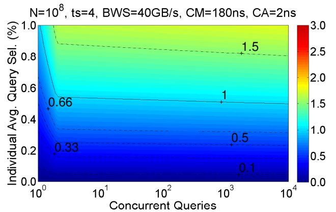
Figure 21: SIMD-aware sorting favors indexing.
