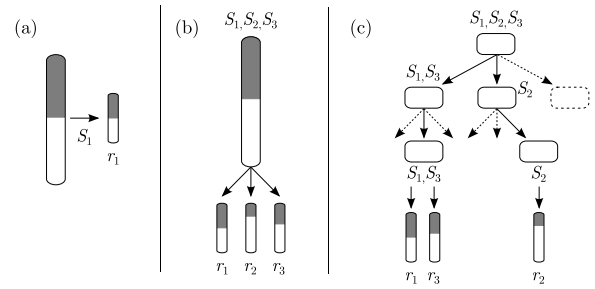
Figure 2: Sequential scan and secondary index scan access patterns of the select operator. Basic scans (a) iterate sequentially through the input and evaluate the predicate to find qualifying positions. Shared scans (b) iterate over the relation only once. Batched B^+ -Tree traversal (c) issues prefetches at each level but only for the children that are needed.
