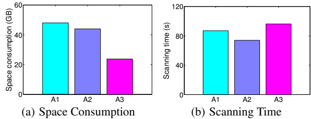
Figure 25: Comparison between table representations.
