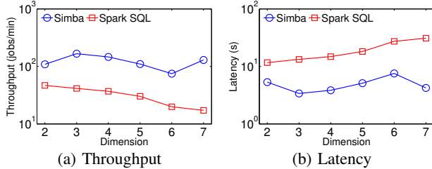
Figure 16: Range query performance on GDEL: dimensionality.
