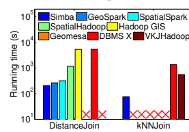
Figure 11: Join operations on different systems.
