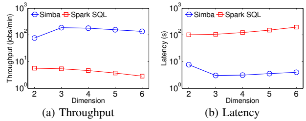
Figure 23: Range query performance on RC: dimensionality.
