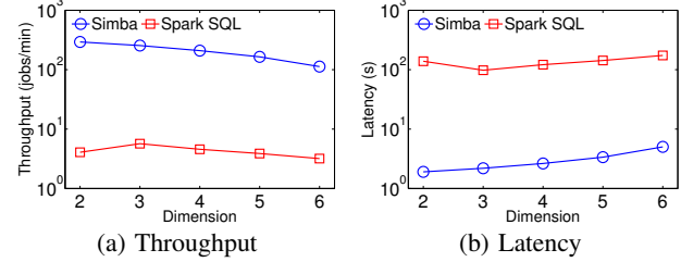
Figure 24: k NN query performance on RC: dimensionality.
