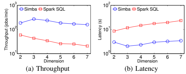
Figure 17: k NN query performance on GDEL: dimensionality.
