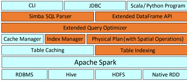
Figure 1: Simba architecture.
