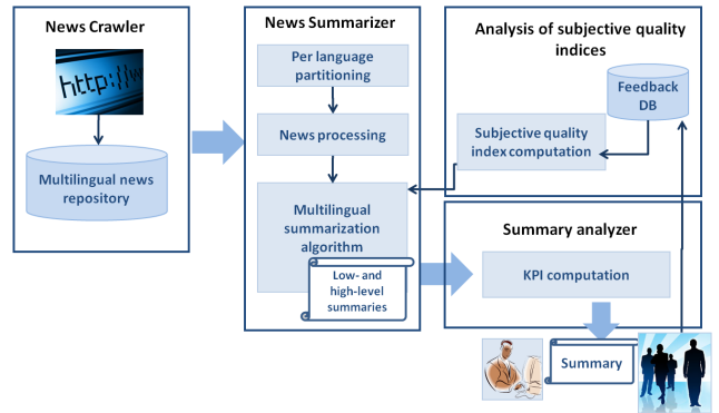
Figure 1: The Stock News Summarizer architecture.
