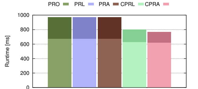
Figure 5: Runtime of PR* vs CPR*-algorithms. Relation sizes: |R| = 128M , |S| = 1280M . Lighter colors denote the partition phase and darker colors denote the join phase.
