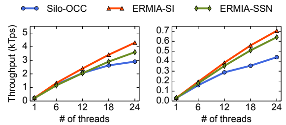
Figure 9: Throughput when running TPC-E-hybrid with 10% AssetEval transaction (left); with 60% AssetEval transaction (right). CC pressure deteriorates scalability of Silo in heterogeneous workloads.
