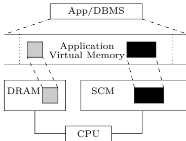
Figure 2: SCM can be mapped directly in the address space of the application.
