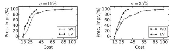
Figure 22: Effects of spammers on cost
