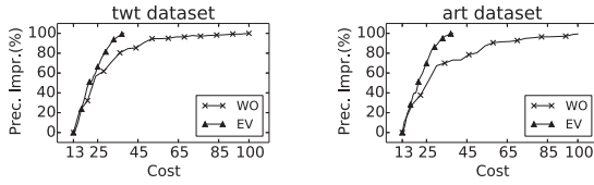
Figure 21: Effect of question difficulty on cost
