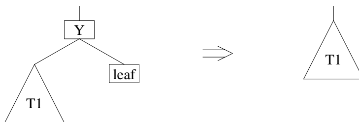
Figure 3.11: Deleting node Y when one subtree is a leaf (easy case)
