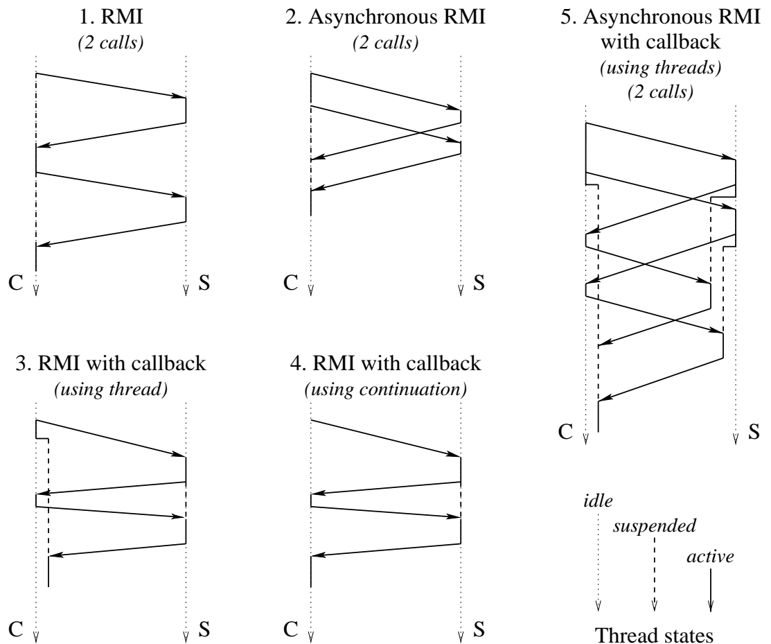
Figure 5.3: Message diagrams of simple protocols
