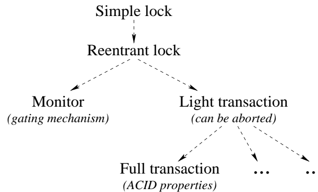
Figure 8.4: The hierarchy of atomic actions
