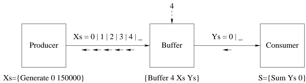
Figure 4.14: Bounded buffer
