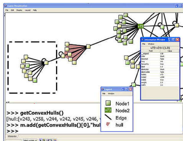
Figure 1: A screenshot of the GUESS system.
