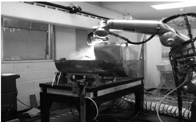
Figure 1. The remote welding testbed used by the group.
