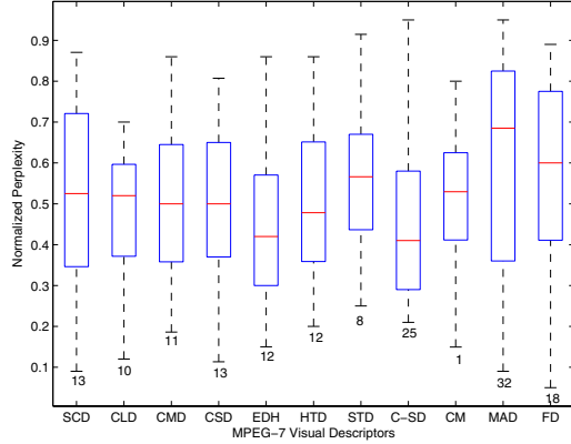
Figure 3: Normalized Perplexity Boxplot.
