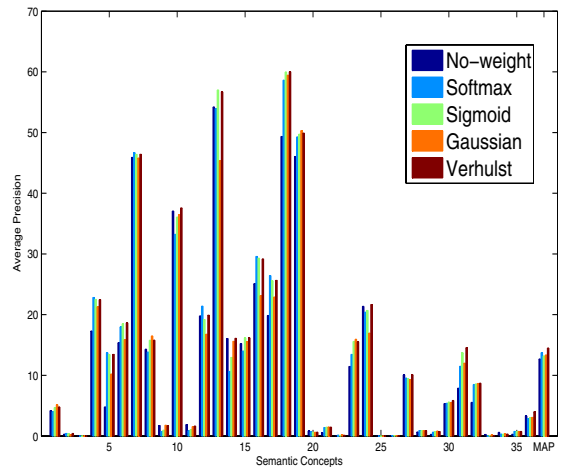
Figure 6: Performance comparison of the 5 approaches across the 36 benchmark concepts on the fusion set. PENN based on Verhulst model outperform all other approaches by a wide weighted combination.
