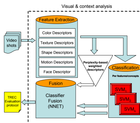
Figure 1: General indexing system architecture.
