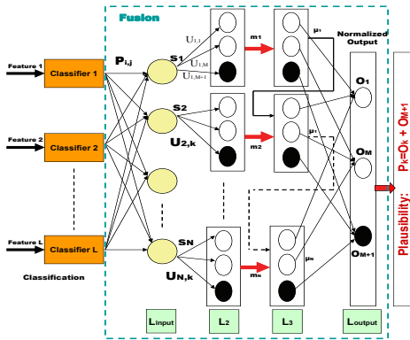
Figure 4: NNET classifier fusion structure.
