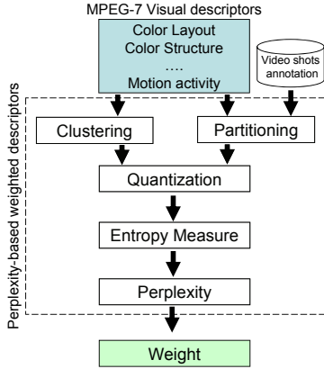
Figure 2: Perplexity-based weighted descriptors structure.
