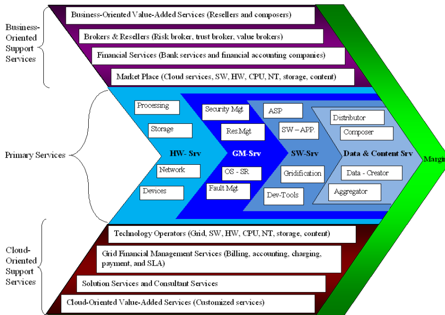
FIGURE 1. Cloud Value Chain Reference Model
