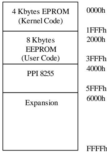
Figure 10. Memory Map of Target System
