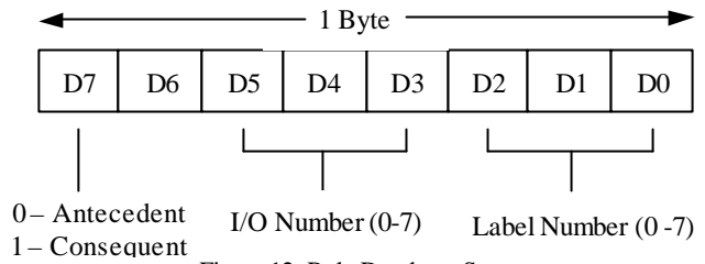
Figure 12. Rule Database Structure
