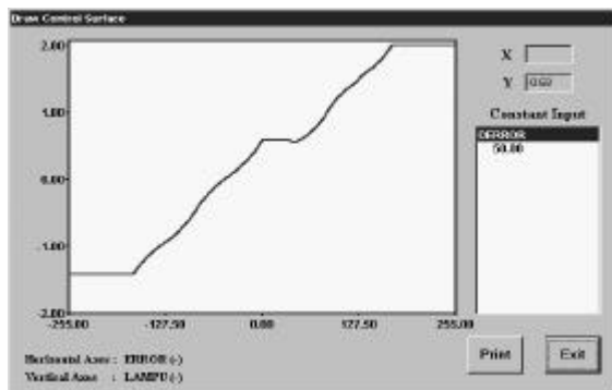
Figure 6. Sample of Graphics From Control Surface
