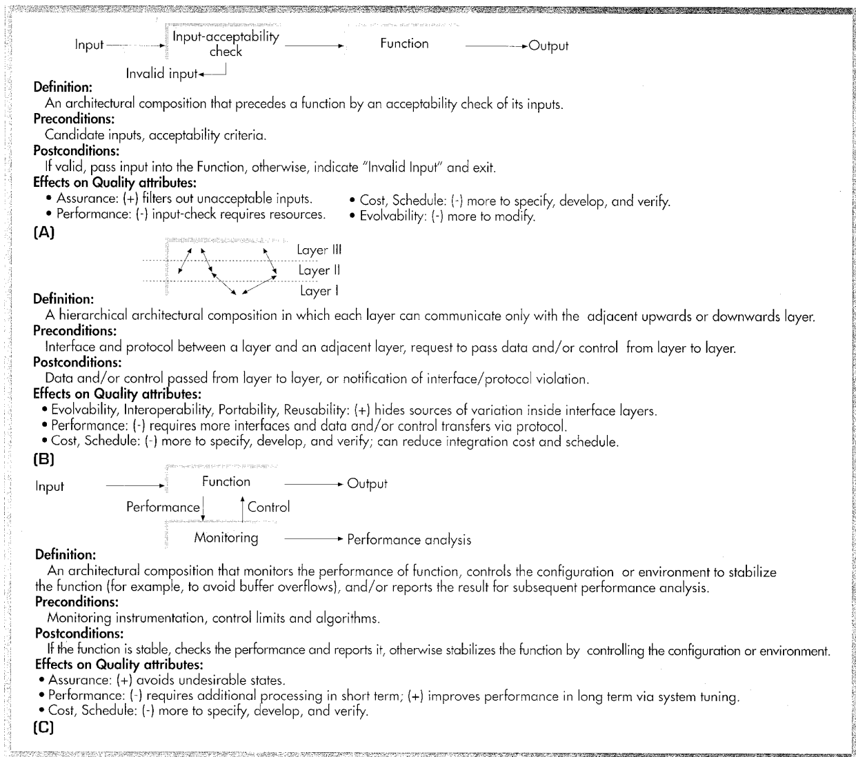
Figure 7. Three examples of primitive quality-attribute architectural strategies: (A) input-acceptability check, (B) layering, and (C) monitoring.
