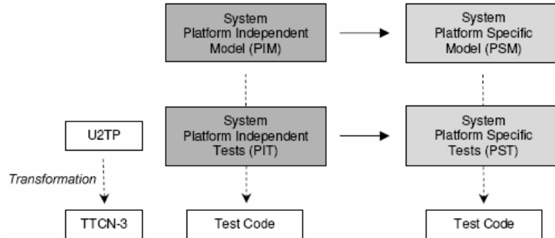
Fig. 4. Test Design Models for U2TP to TTCN-3 Transformation Approach
