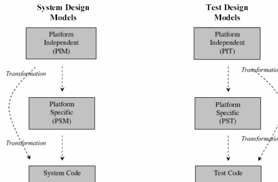
Fig. 1. System Design Models versus Test Design Models
