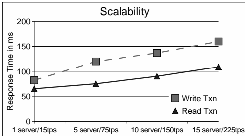
Figure 5: Response time for update transactions and queries
