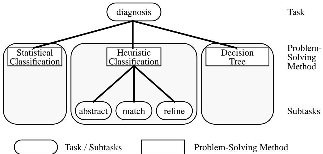
Fig. 3 Sample Task Structure for Diagnosis
